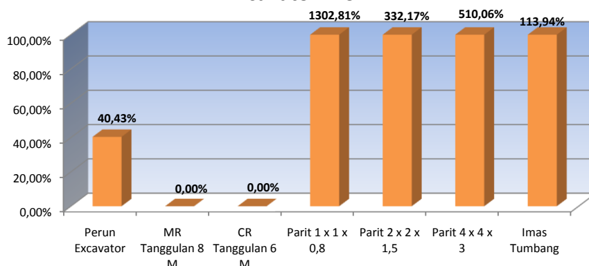
Excavator Work
